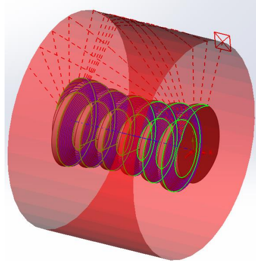
Clearance Type set to 'Cylinder about X'
