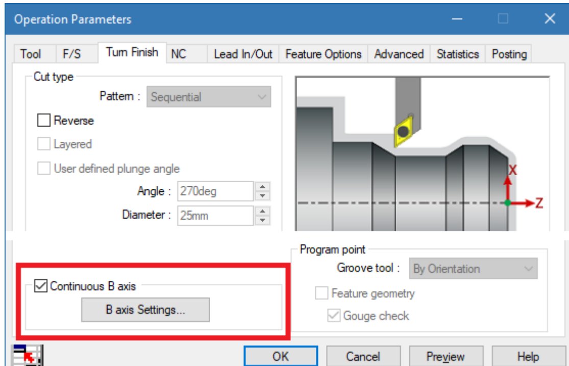
'Continuous B Axis' group box in Turn Finish Tab for a Turn Finish Operation
