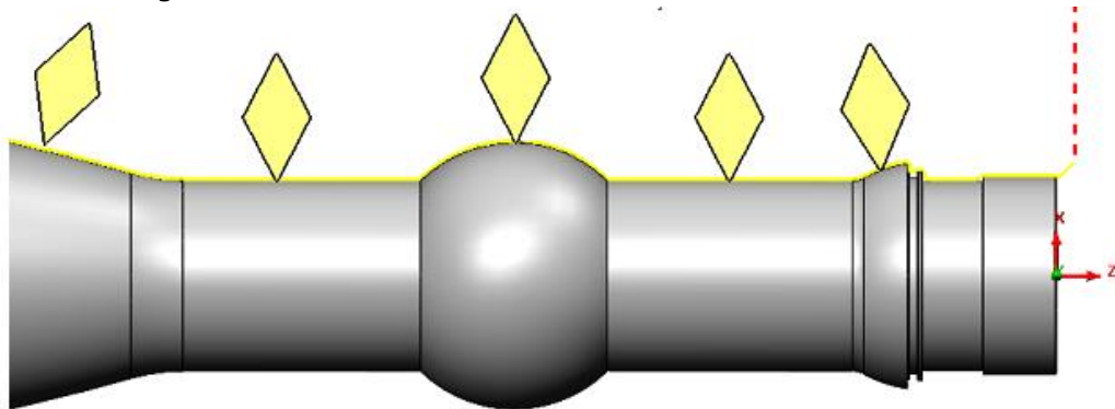
Image illustrating how Continuous B Axis Turning functionality works when the Type of Cut for the toolpath is set to 'At an Angle to the Feature Curve'
