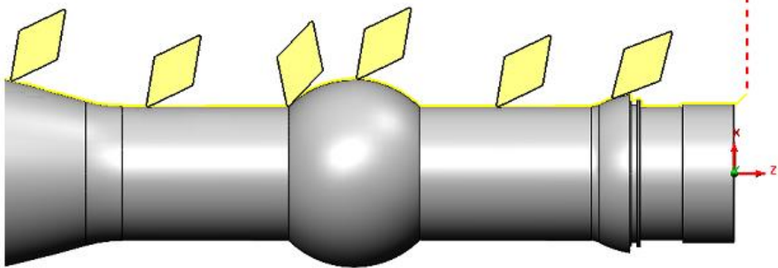
Image illustrating how Continuous B Axis Turning functionality works when the Type of Cut for the toolpath is set to 'Constant Angle'
