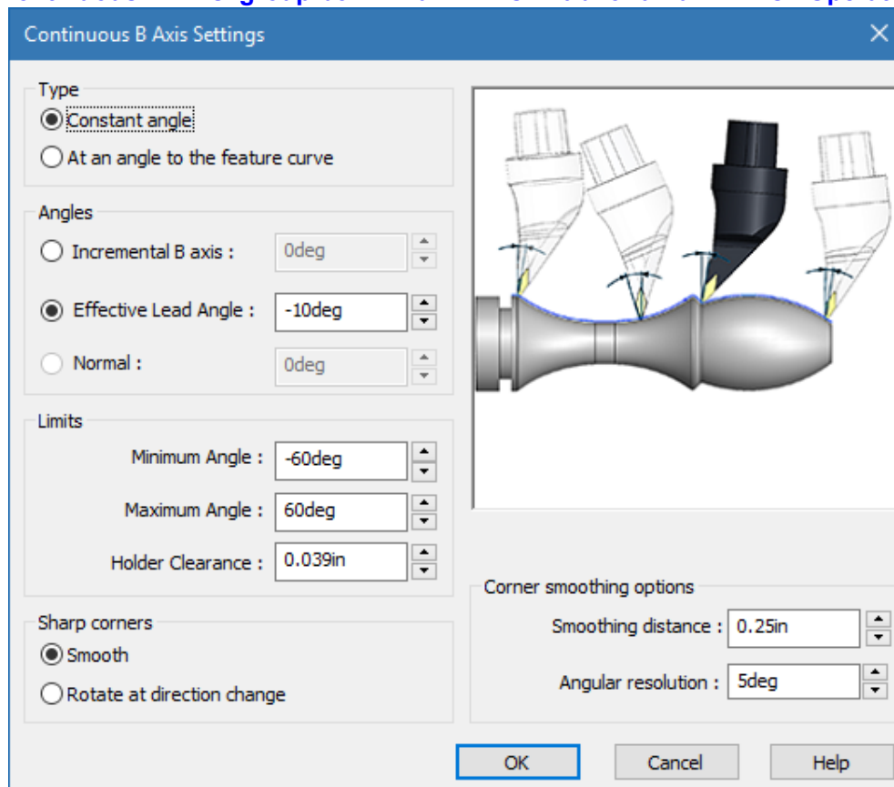
'Continuous B Axis Settings' Dialog Box
