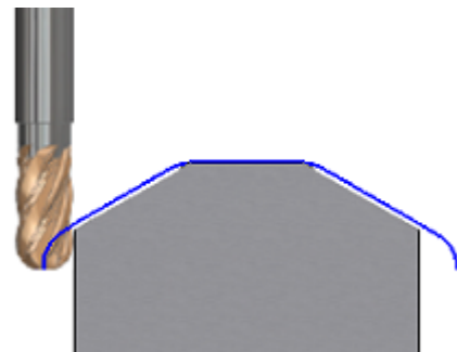
Toolpath when "Waterfall Ends" option is checked
