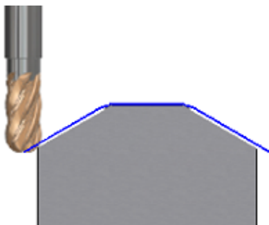
Toolpath when “Waterfall Ends” option is unchecked
