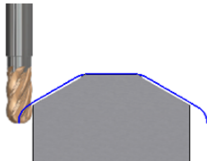
Toolpath when “Waterfall Ends” option is checked
