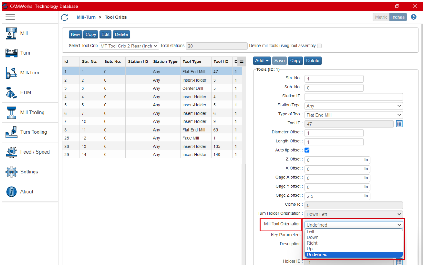
New 'Mill Holder Orientation' Parameter in Tools Form of Mill-Turn Tools Cribs UI
